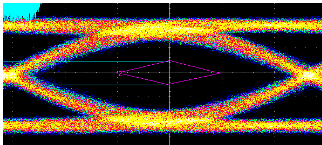
18Gbps Eye Pattern
