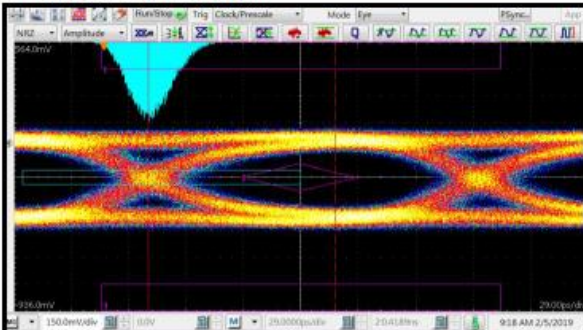
UHDV 30 meter EYE & I2C:
