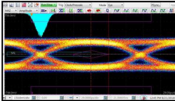
UHDV 50 meter EYE & I2C:
