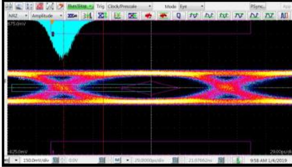
UHDV 10 meter EYE & I2C:
