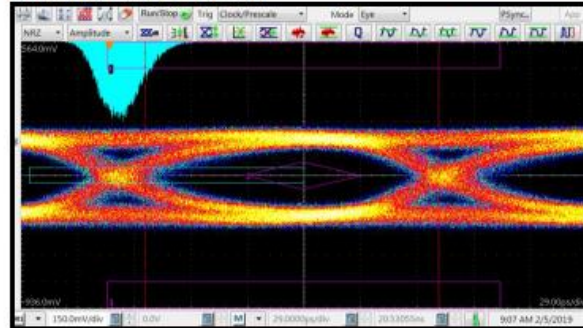
UHDV 20 meter EYE & I2C:
