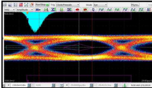
UHDV 40 meter EYE & I2C:
