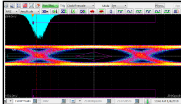
UHDV 15 meter EYE & I2C:
