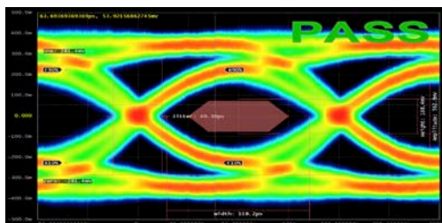
18Gbps Eye Pattern
